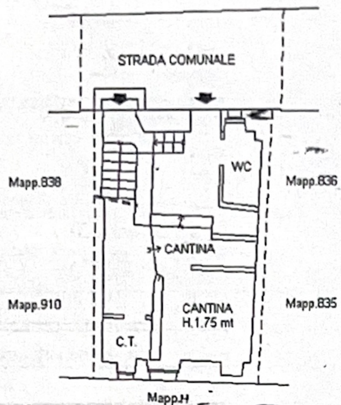
PIANO TERRA H.2.65 mt.
